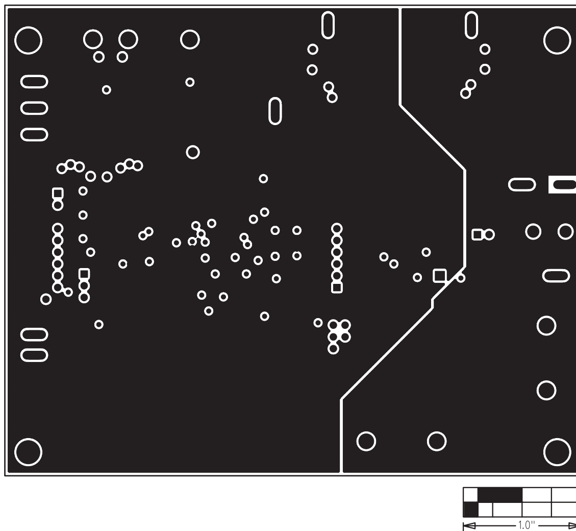
Figure 18. MAX9850 EV Kit PCB Layout—Inner Layer 2
