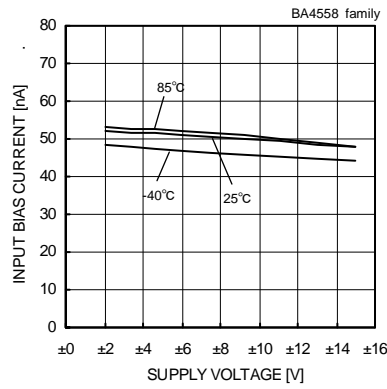
Fig. 11 Input Bias Current - Supply Voltage (Vcm=0[V], Vout=0[V])
