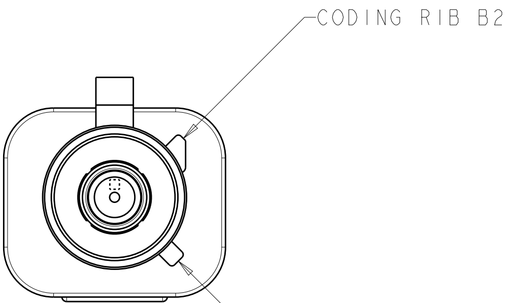
DETAIL H SCALE 5:1
