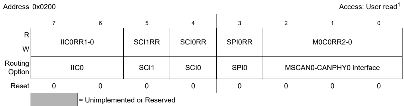
Figure 2-1. Module Routing Register 0 (MODRR0)
