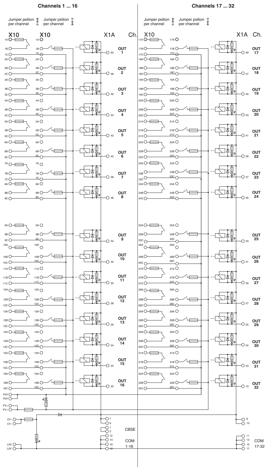
Circuit diagram
