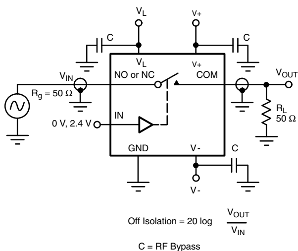
Fig. 6 - Off-Isolation
