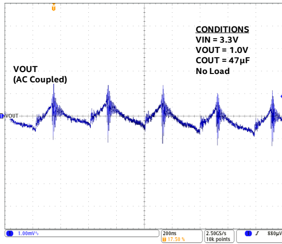
Buck Output Voltage Ripple
