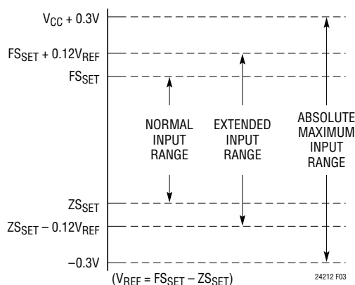
Figure 3. LTC2421/LTC2422 Input Range
