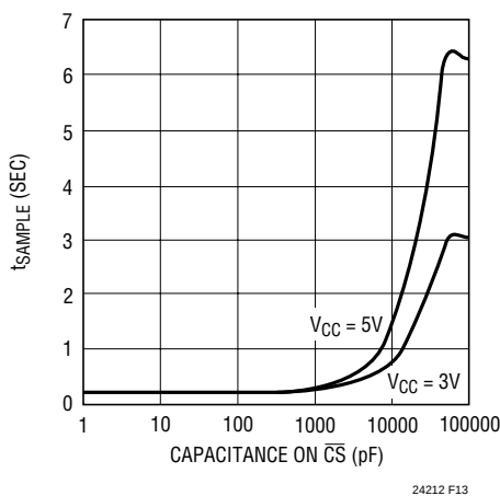
Figure 13. \overline{\text{CS}} Capacitance vs t SAMPLE
