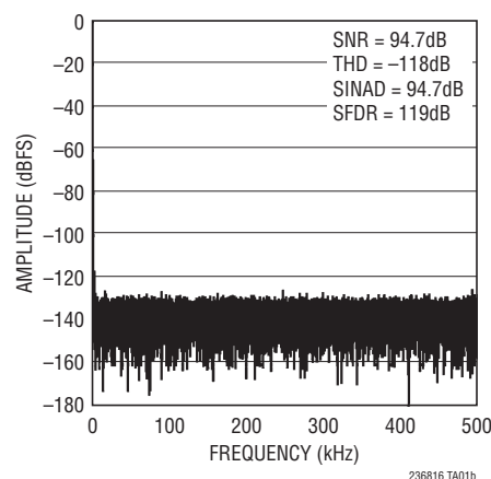
32k Point FFT f_{\text{S}} = 1\text{Msps} , f_{\text{IN}} = 2\text{kHz}
