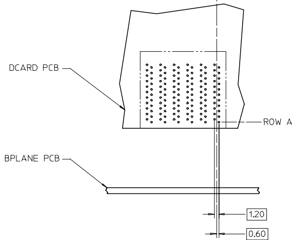
36 PAIR ORTHOGONAL MIDPLANE NODE (USES TWO 6 COLUMN I-TRAC HEADERS)
