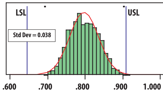
Figure 1. I_{ds} ; LSL = 640mA, nominal = 800mA, USL = 910mA
