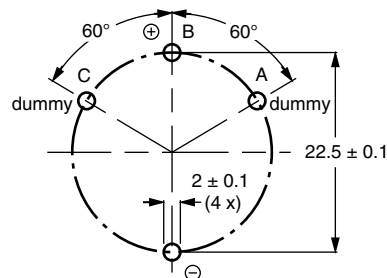
Fig. 3 - Mounting hole diagram
