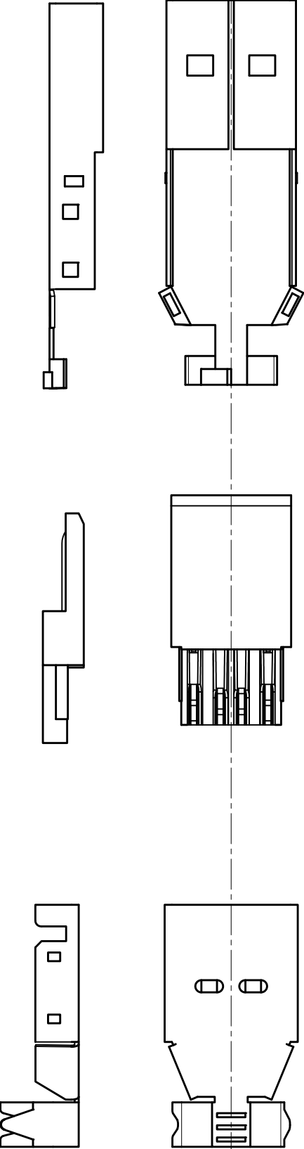
FRONT SHELL
