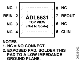
Figure 2. Pin Configuration
