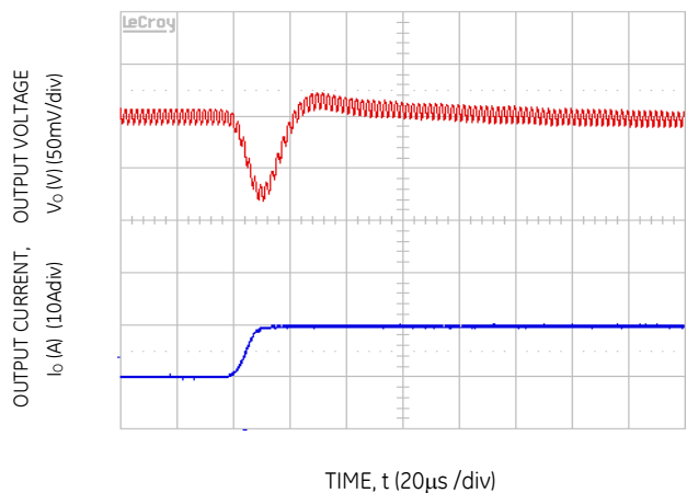
Figure 34. Transient Response to Dynamic Load Change from 50% to 100% at 12Vin, Cout= 8x47uF, CTune=1500pF & RTune=220 ohms
