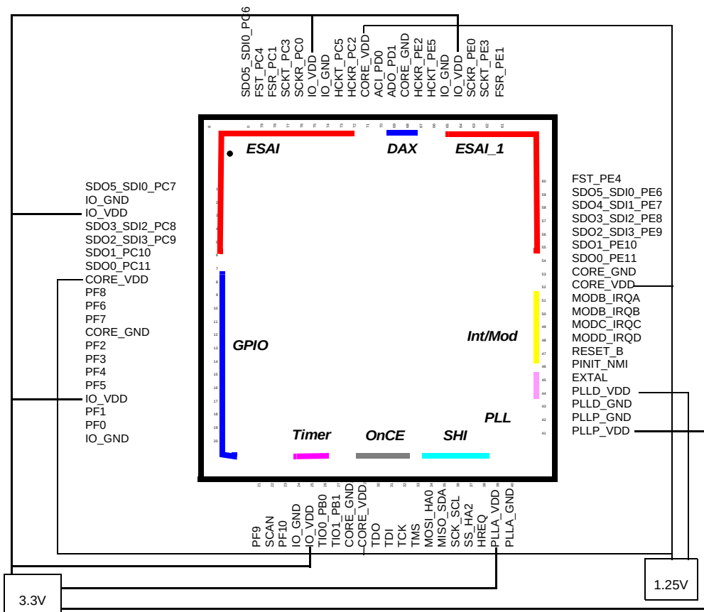
Figure 3. VDD Connections
