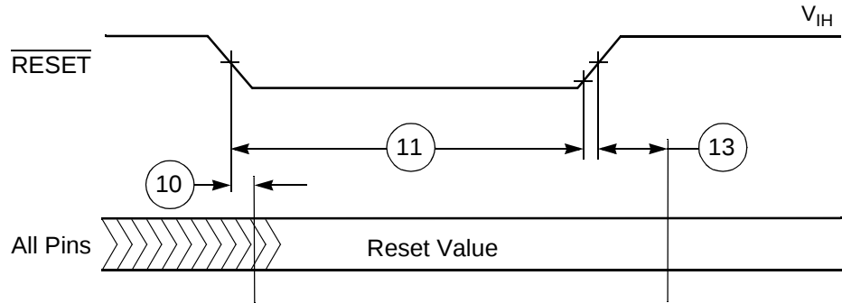
Figure 5. Reset Timing
