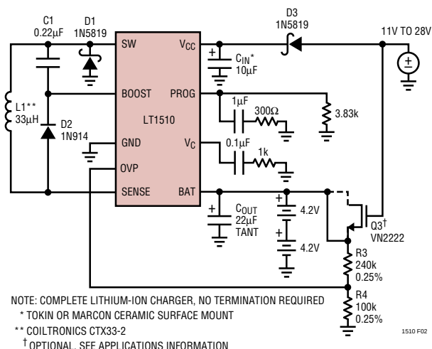
Figure 2. Charging Lithium Batteries (Efficiency at 1.3A > 87%)
