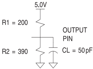
Figure 3-3. Output Test Loads
