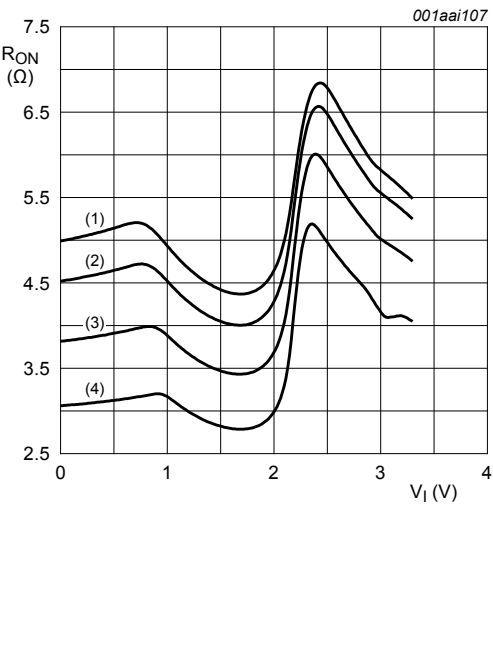
Fig. 14. ON resistance as a function of input voltage; V_{CC} = 3.3 V; I_{SW} = 64 mA
