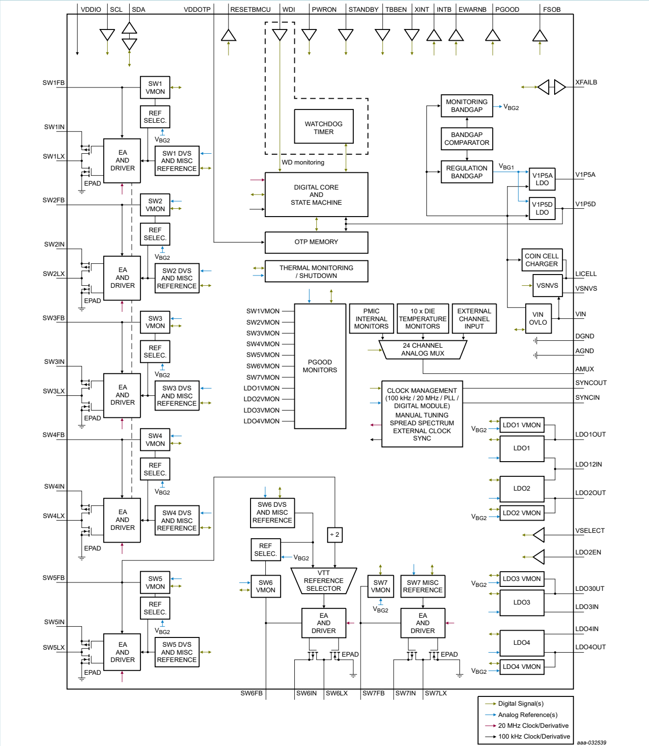
Figure 2. Internal block diagram
