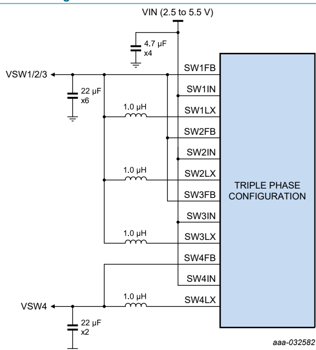
Figure 26. Triple phase configuration
