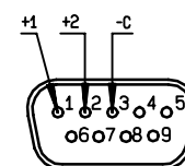
D-SUB 9 PINS TOP VIEW
