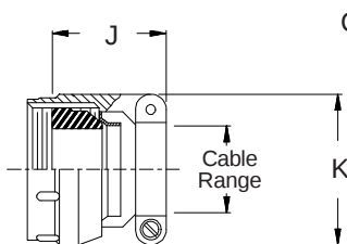
STYLE C Medium Duty (Table IV)
