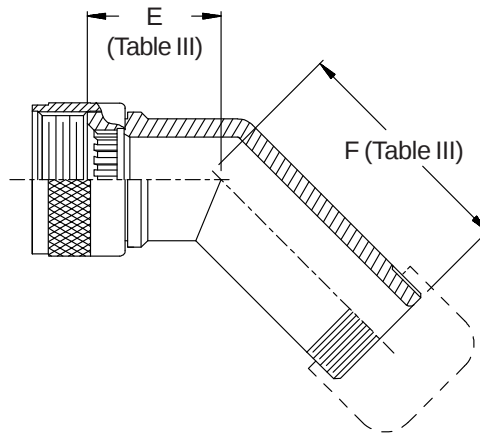
STYLE C Medium Duty (Table IV)
