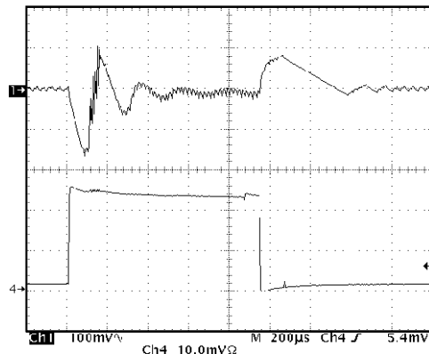
250 - mA Transient 12 V Converter (V IN = 10 V)
