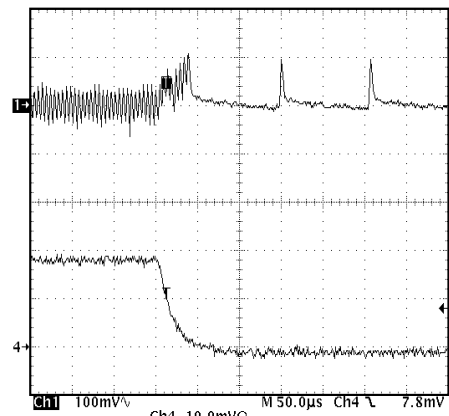
PWM → PSM 3 V Converter (V IN = 10 V)
