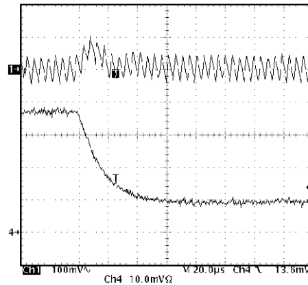
PWM, Unloading 3 V Converter (V IN = 10 V)
