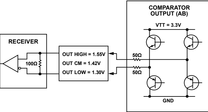
Figure 82. Comparator Output Scheme
