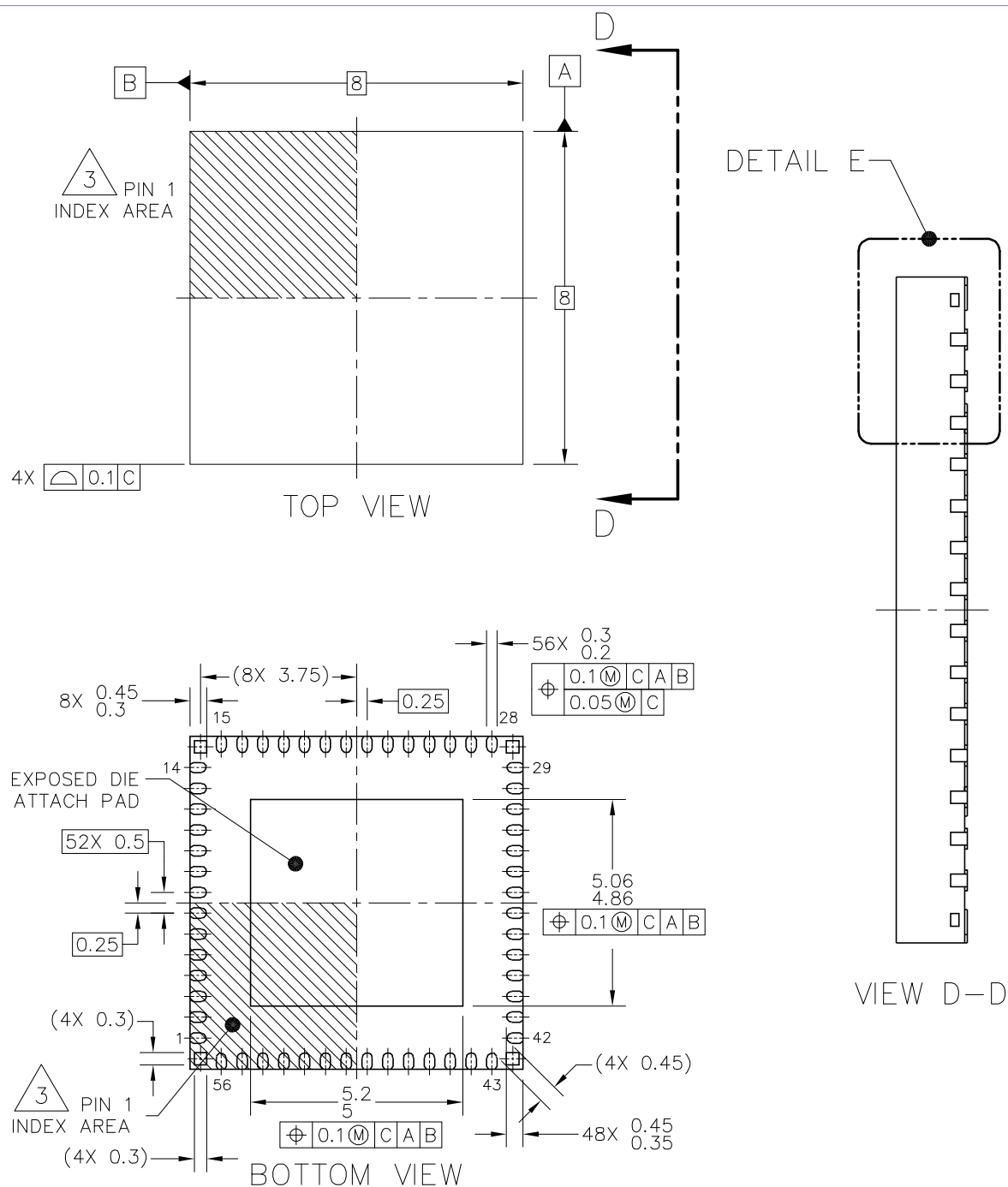
Figure 45. Package outline for E-type HVQFN56 (Industrial grade)
