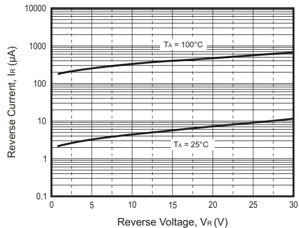
Fig.6 - Reverse Characteristics
