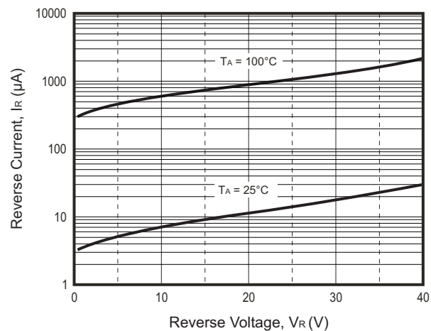
Fig.8 - Reverse Characteristics
