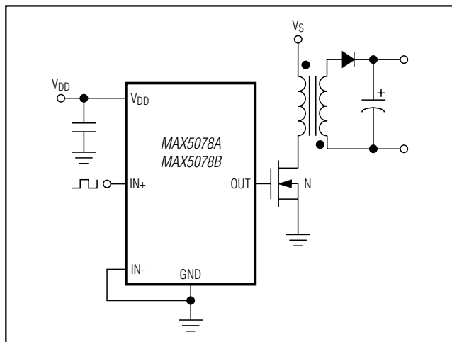
Figure 4. Noninverting Application
