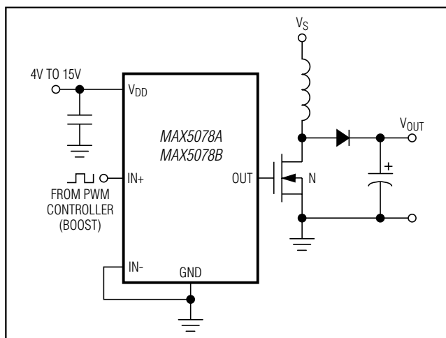
Figure 5. Boost Converter
