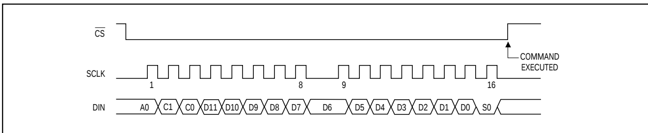
Figure 5. Serial-Interface Timing Diagram
