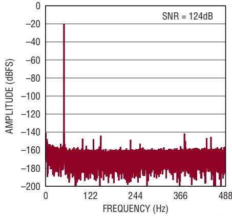
32k Point FFT f_{SAMPL} = 1\text{Msps} , f_{IN} = 50\text{Hz} , N = 1024
