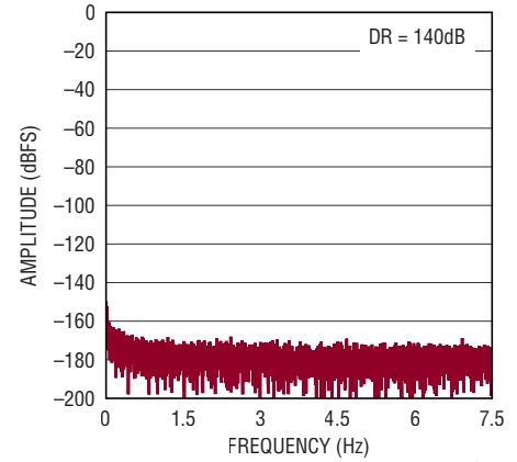
8k Point FFT f_{SAMPL} = 1\text{Msps} , IN^+ = \text{Near GND} , IN^- = \text{GND} , N = 65536
