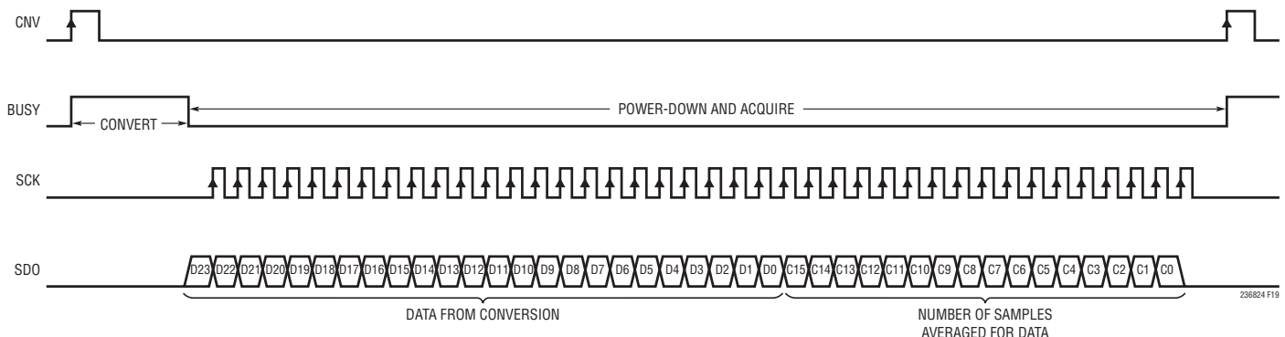
Figure 19. Serial Output Code Parsing
