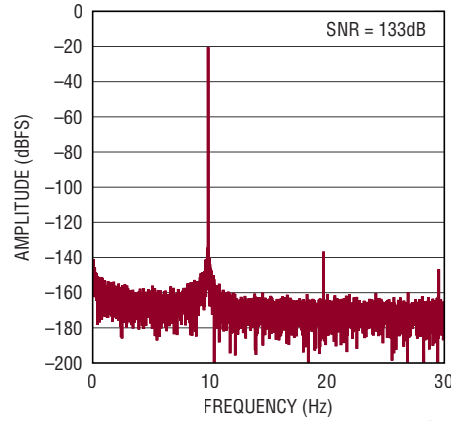
32k Point FFT f_{SAMPL} = 1\text{Msps} , f_{IN} = 10\text{Hz} , N = 16384
