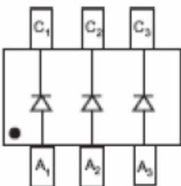
MBD4448HTW
