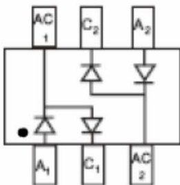
MBD4448HSDW
