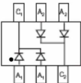
MBD4448HCDW
