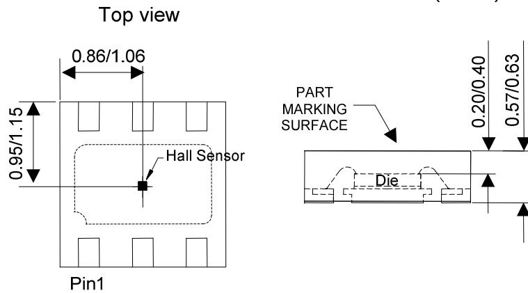
Sensor Location (TBD)
