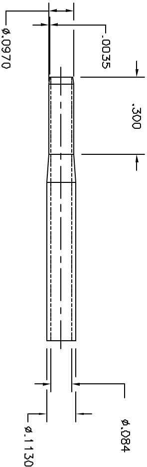
PROBE DETAIL
