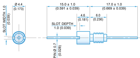
6-32 UNC Class 2A Thread 4.4mm Round Head
