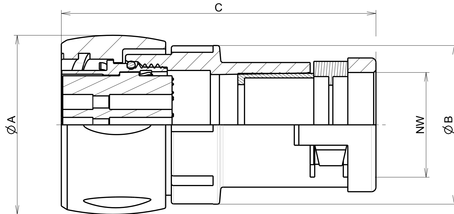
ASSEMBLED VIEW
