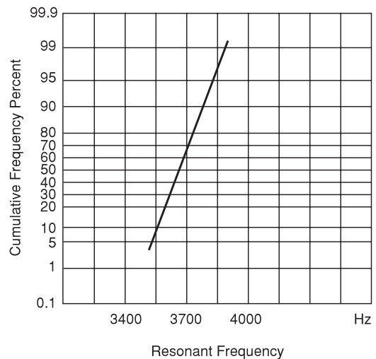
(4) Resonant Frequency
