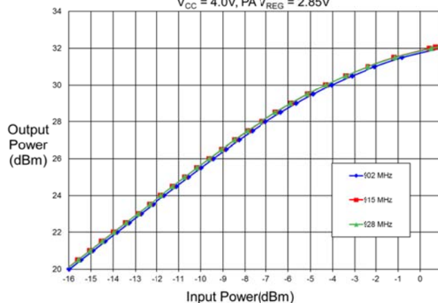
Input Power versus Output Power V_{CC}=4.0V , PA V_{REG}=2.85V
