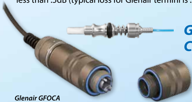
Glenair GFOCA hermaphroditic fiber optic connection system is optimized for rapid deployment in rugged field applications.
