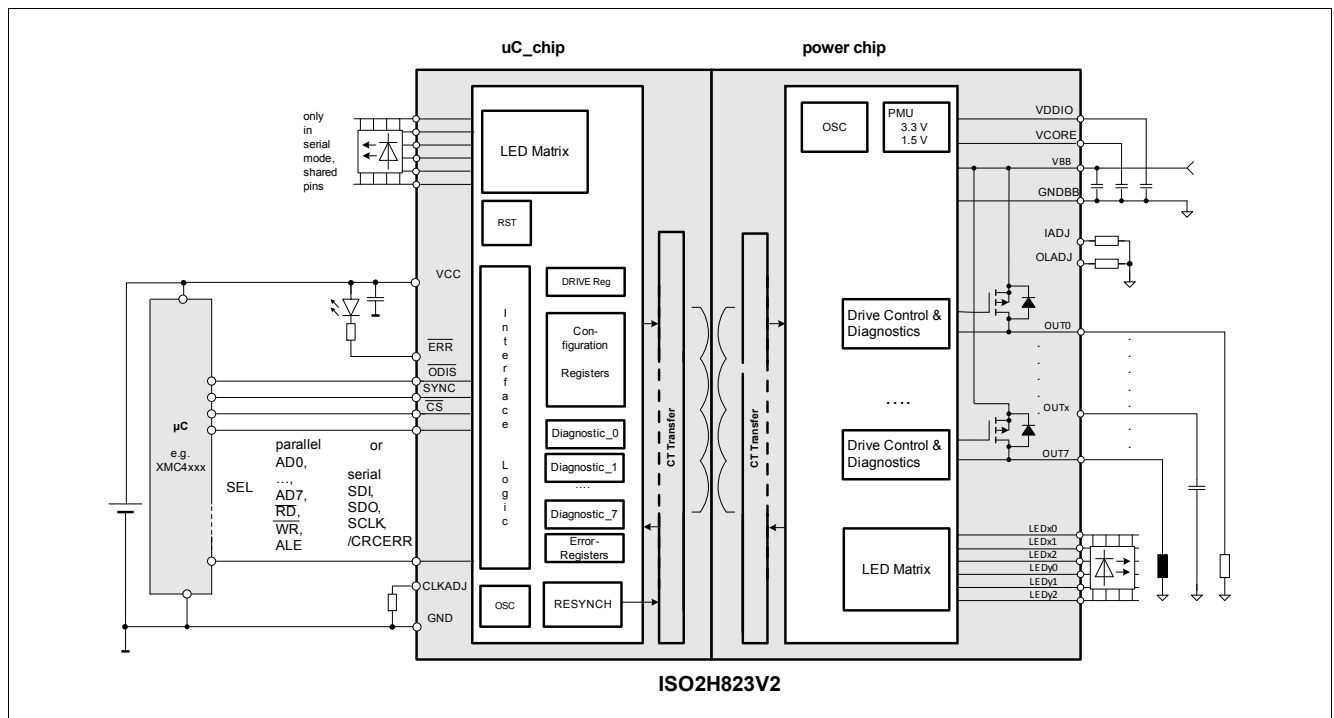
Figure 1 Typical Application
