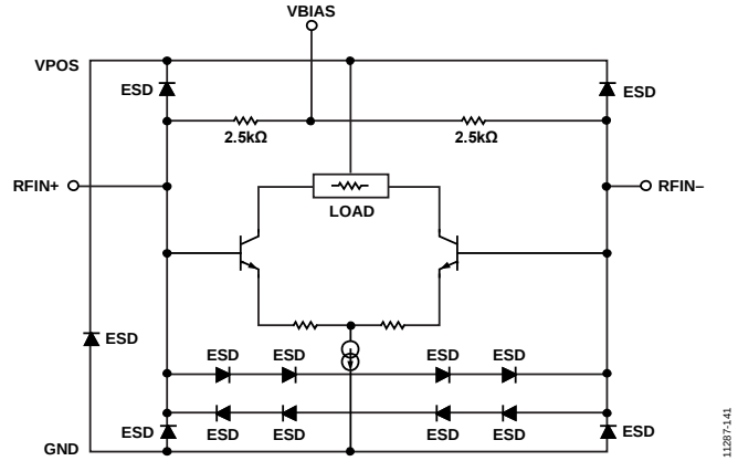
Figure 42. RF Inputs
