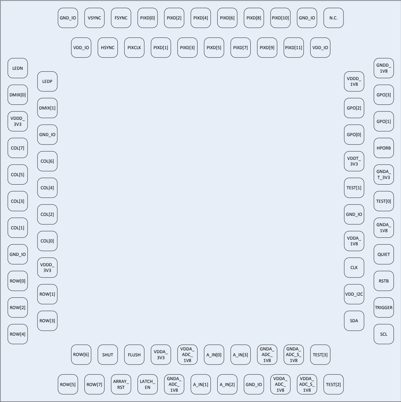
Figure 4: Array QFN package, 84 pins. Top view.
