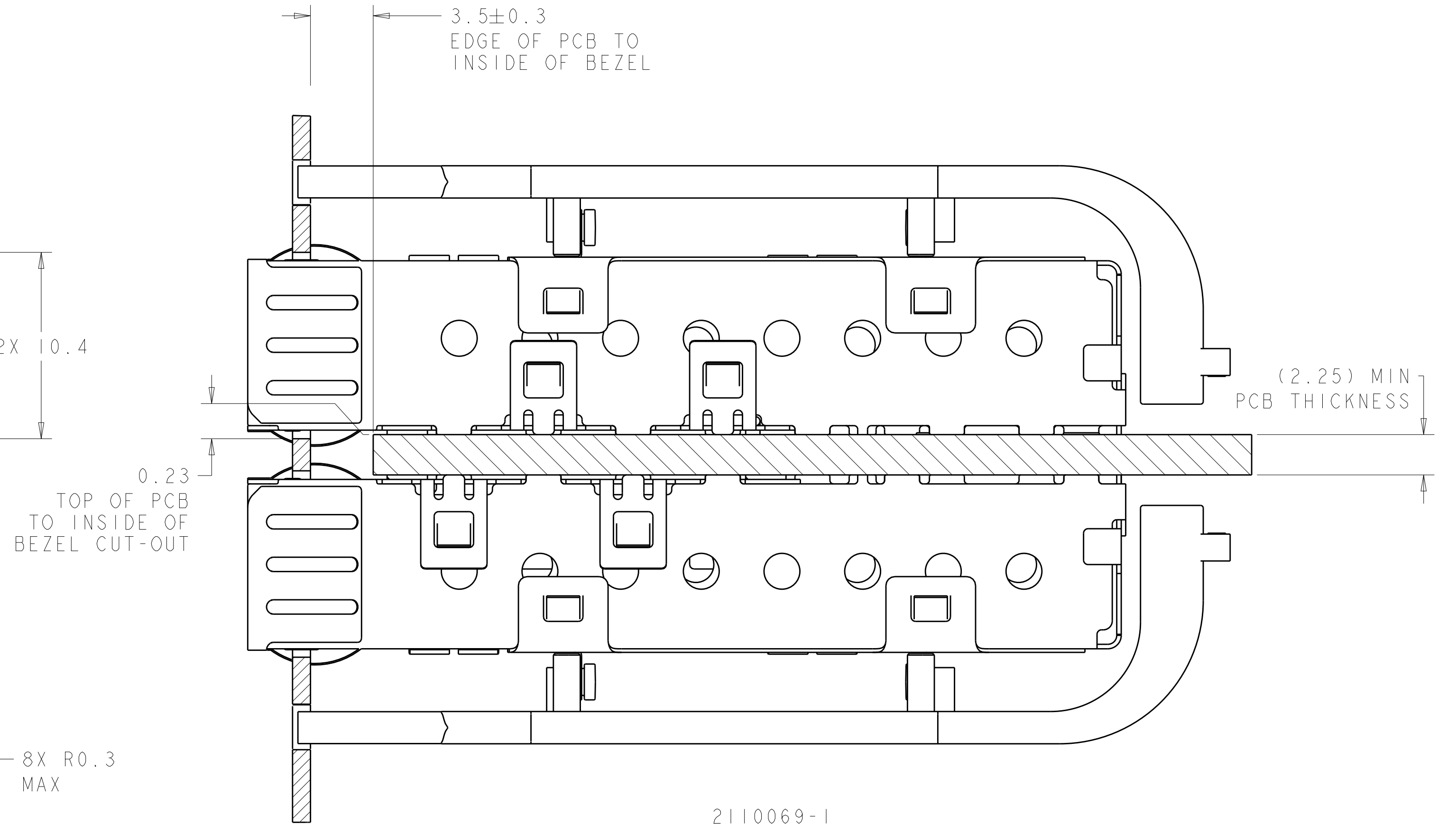
2110069-1 MOUNTED BELLY TO BELLY ON PC BOARD SHOWN THRU RECOMMENDED BEZEL
