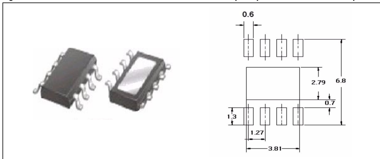
Figure 15: PowerSO-8 with its minimum recommended footprint (all dimension are in mm)
