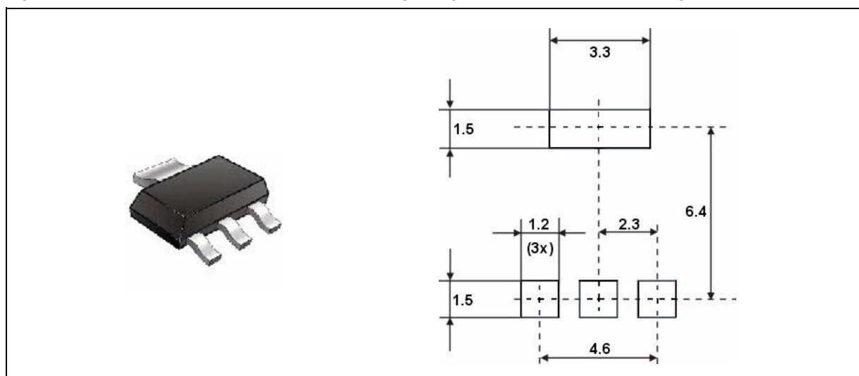
Figure 8: SOT-223 and its recommended footprint (all dimensions are in mm)
