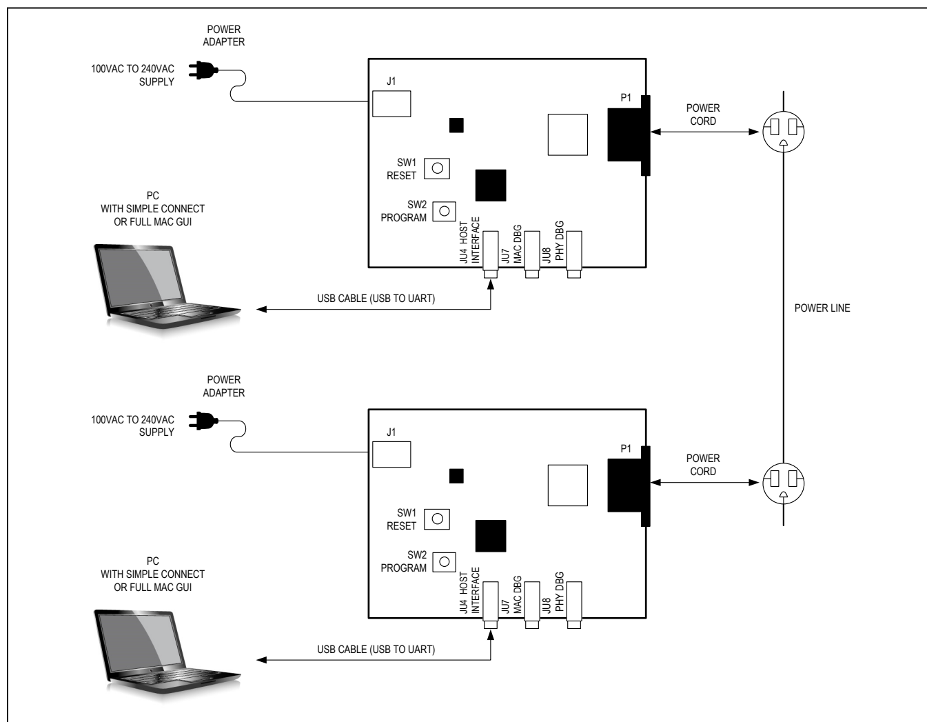
Figure 2. Connection Diagram
