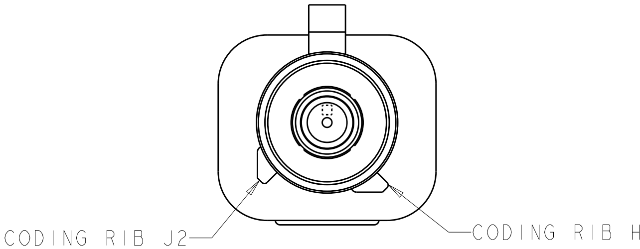
DETAIL M SCALE 5:1
