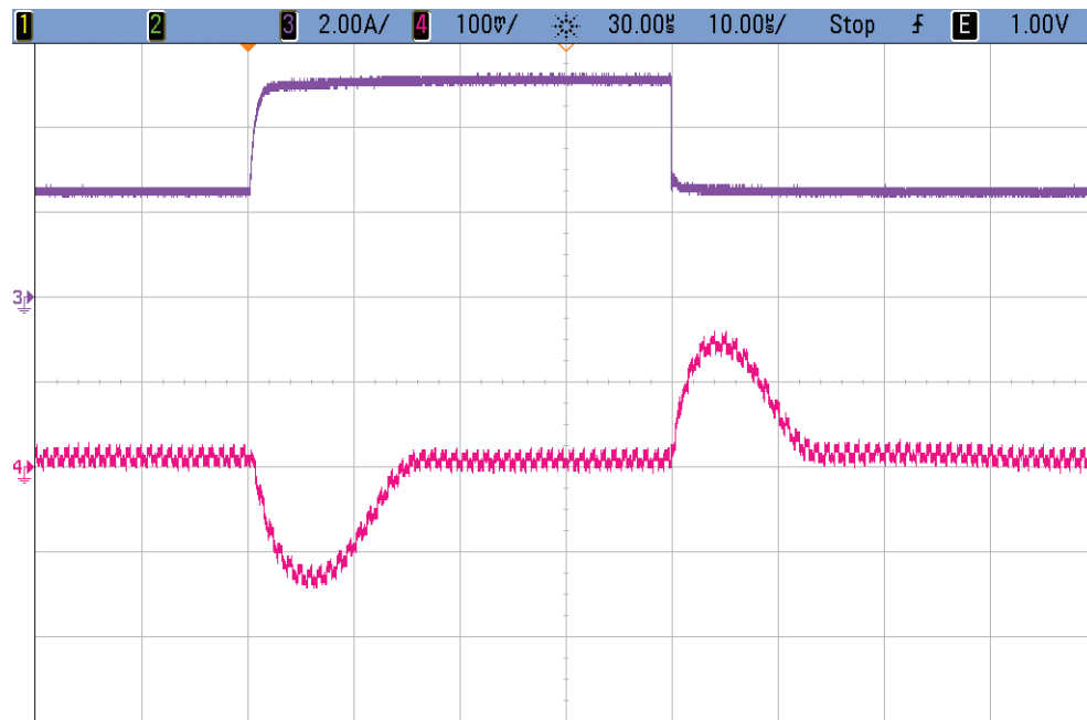
Figure 4. Transient Response Waveform at 12V_{IN} , 5V_{OUT} and 2.5 - 5 - 2.5A_{OUT} (2A, 100mV, 10\mu s/DIV , 20MHz Bandwidth)
