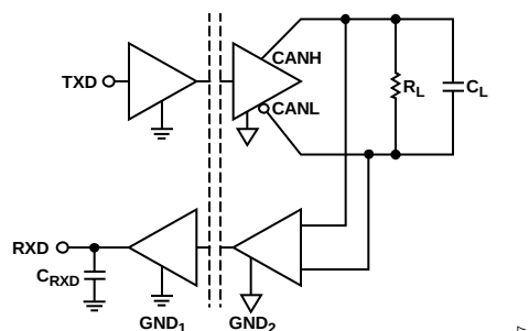
Figure 20. Switching Characteristics Measurements
