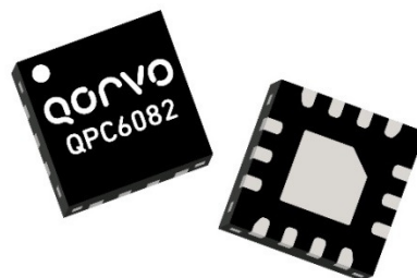
14 Pad 2.0 mm x 2.0 mm x 0.55 mm QFN Package
