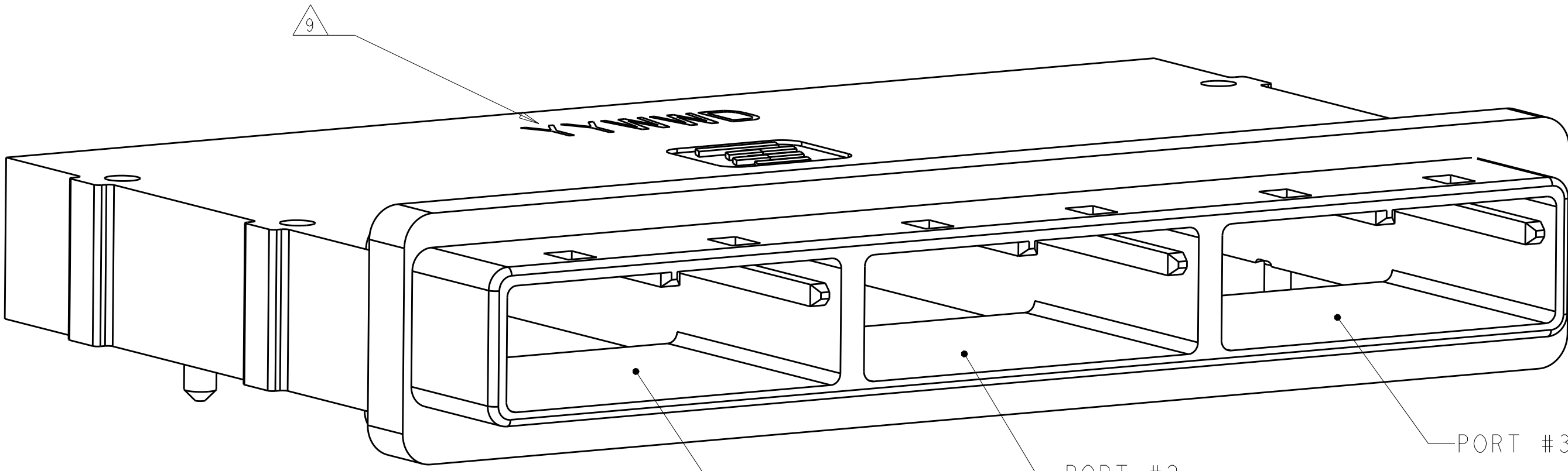
1888321-3 SCALE 5:1
